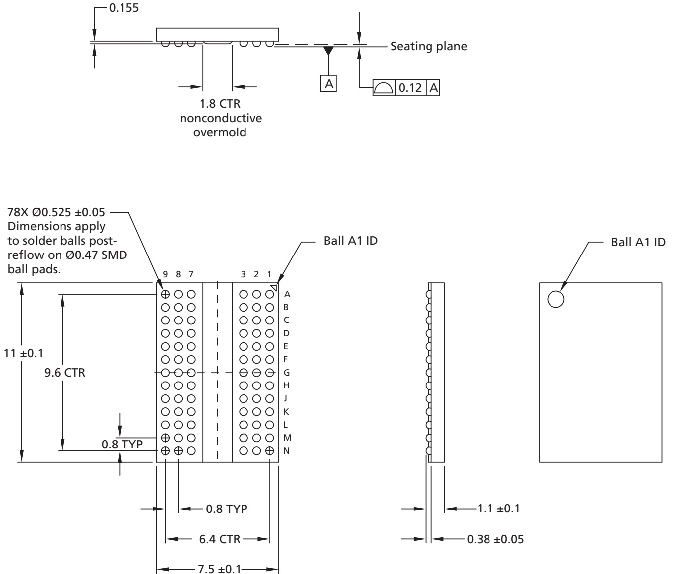
Figure 8: 78-Ball FBGA – x8 (AG)
