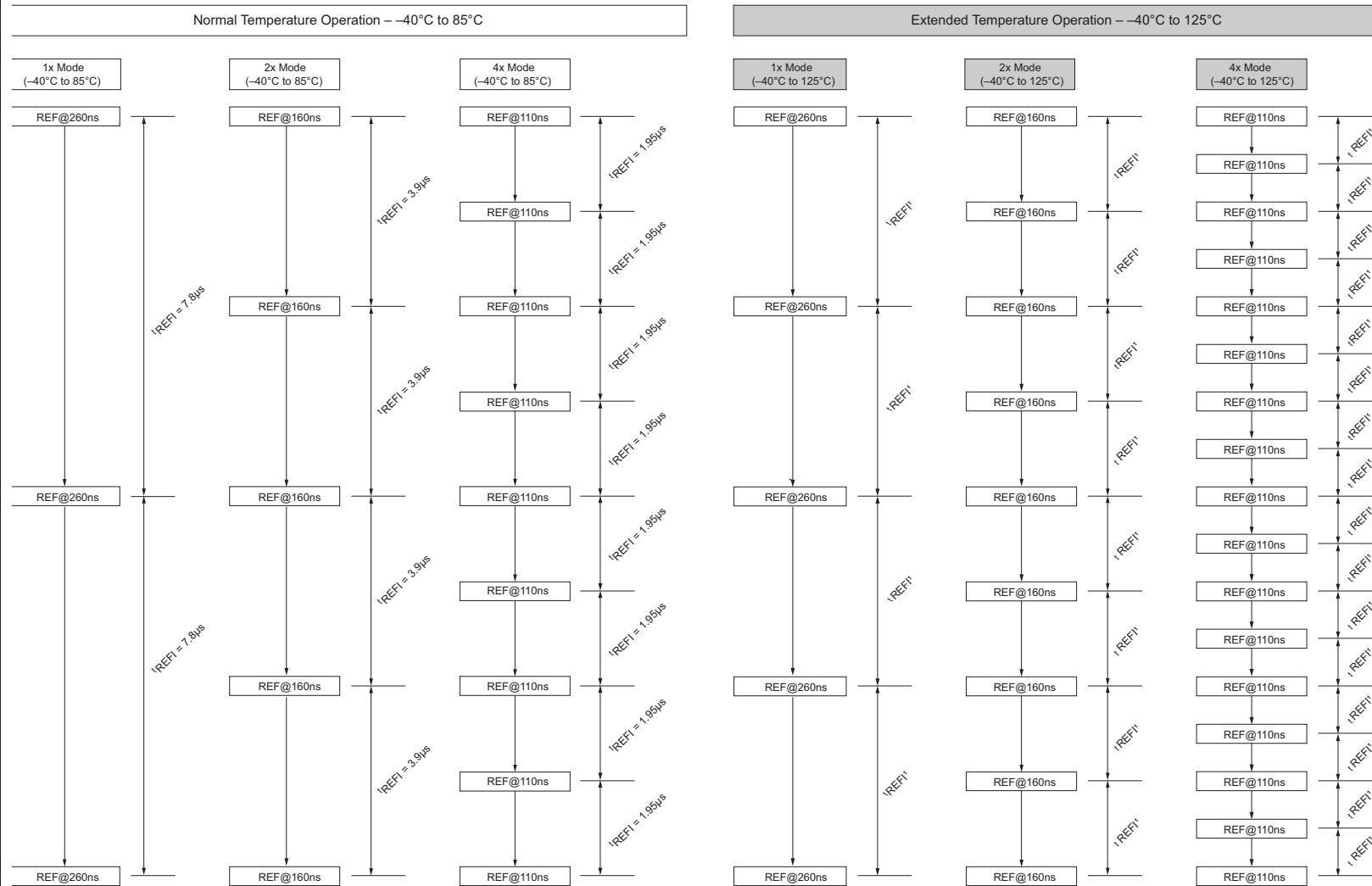
Figure 87: 4Gb with Fine Granularity Refresh Mode Example
