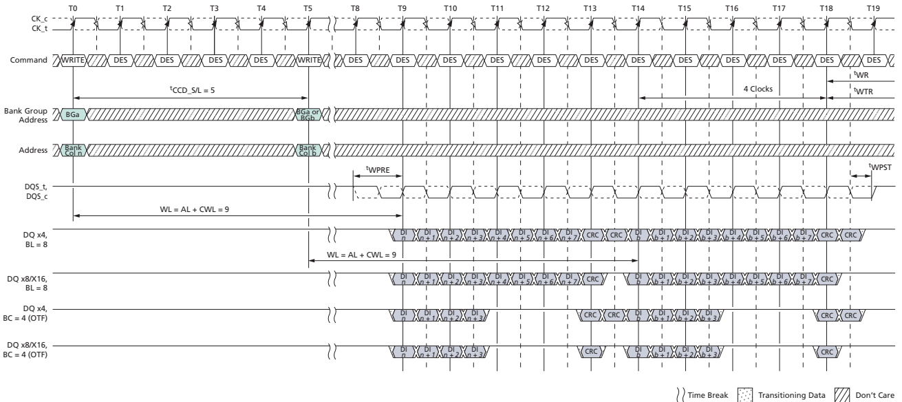
Figure 196: Consecutive WRITE (BL8/BC4-OTF) with 1 st CK Preamble and Write CRC in Same or Different Bank Group
