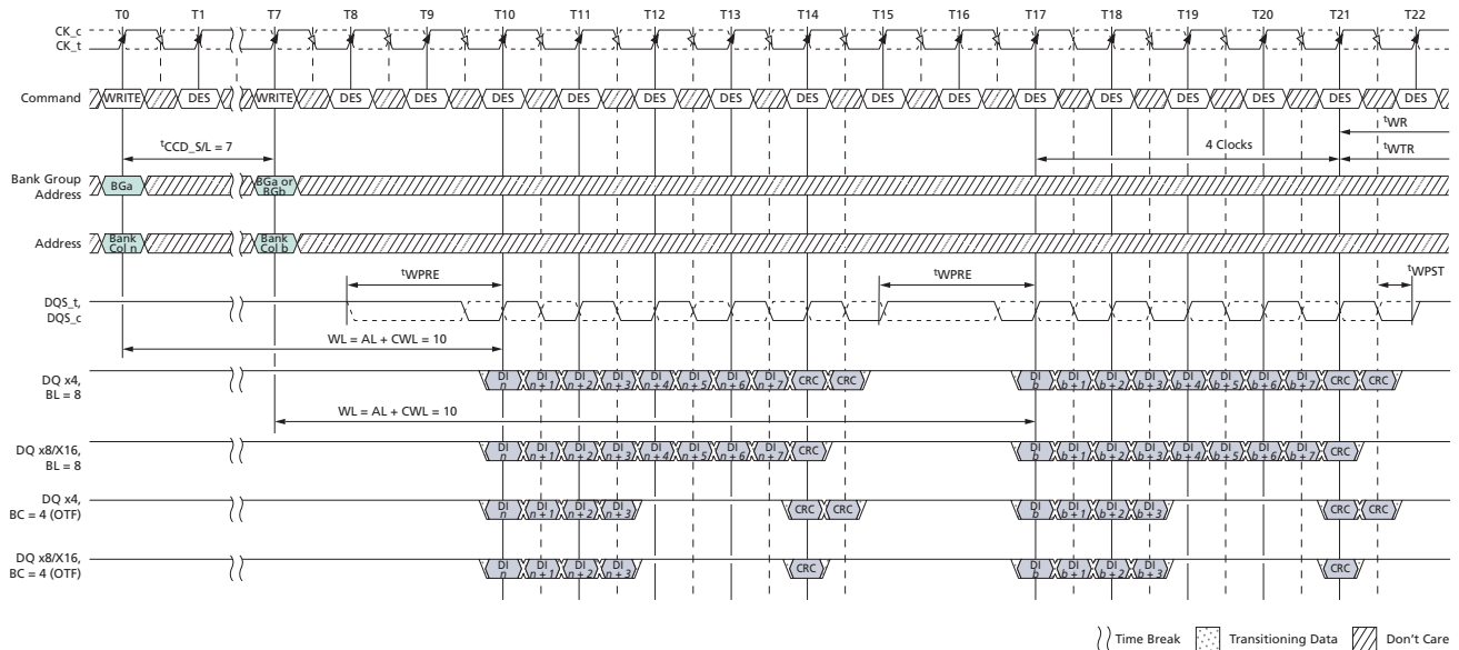
Figure 199: Nonconsecutive WRITE (BL8/BC4-OTF) with 2^t\text{CK} Preamble and Write CRC in Same or Different Bank Group
