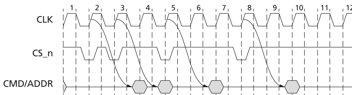
Figure 26: CAL Timing Example (Consecutive CS_n = \text{LOW} )
