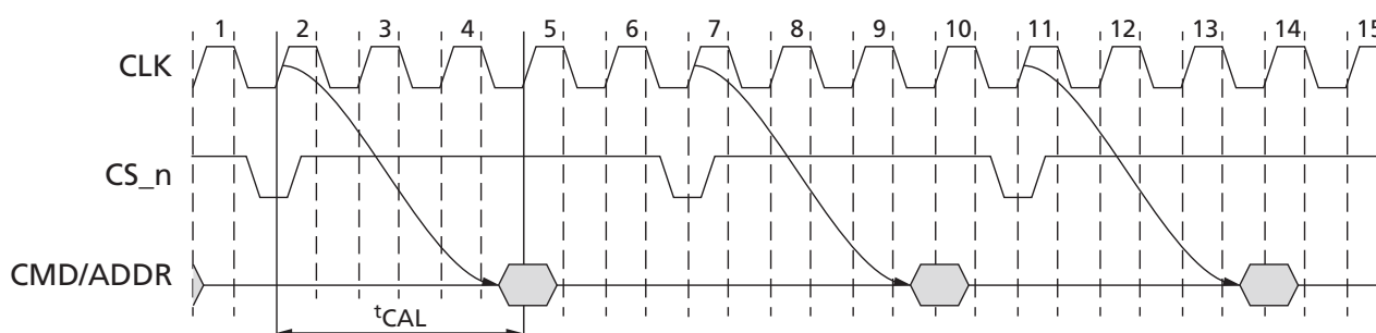
Figure 25: CAL Timing Definition
