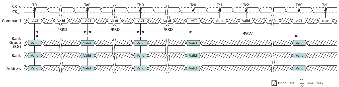
Figure 82: t_{FAW} Timing
