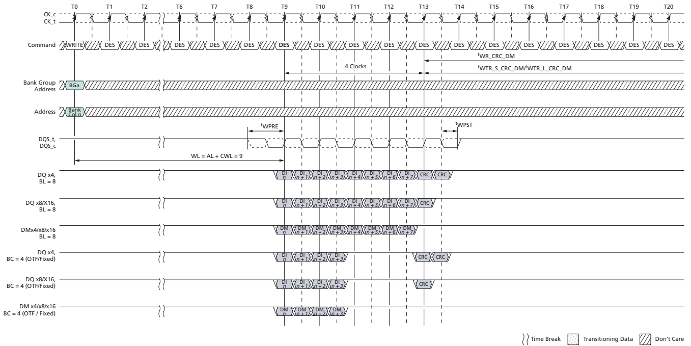
Figure 200: WRITE (BL8/BC4-OTF/Fixed) with 1 st CK Preamble and Write CRC in Same or Different Bank Group
