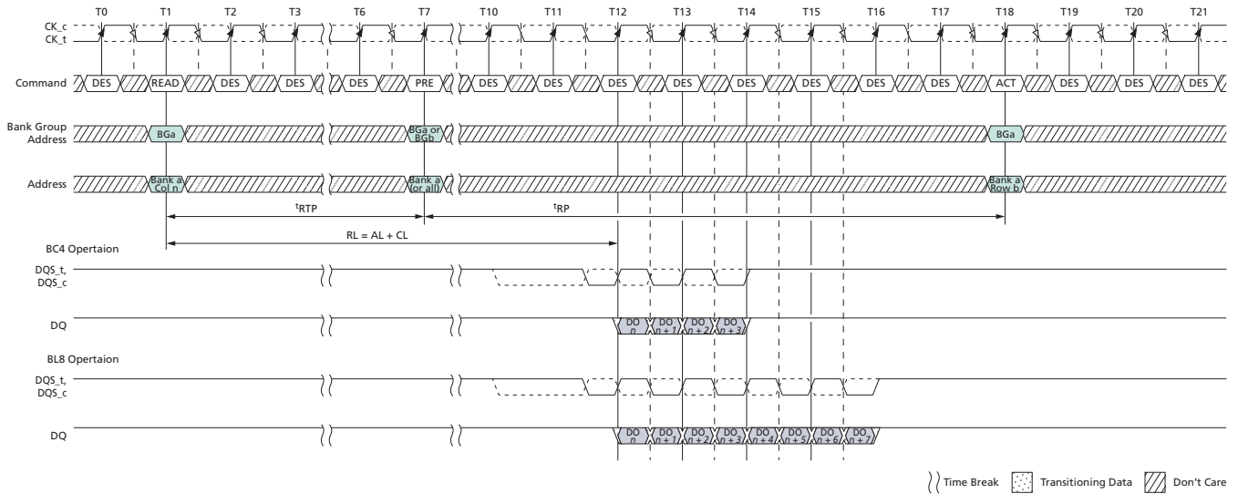
Figure 153: READ to PRECHARGE with 2^t\text{CK} Preamble
