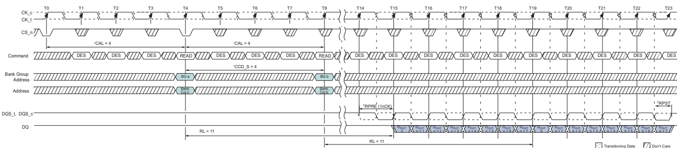
Figure 32: Consecutive READ BL8, CAL4, 1 st CK Preamble, Different Bank Group
