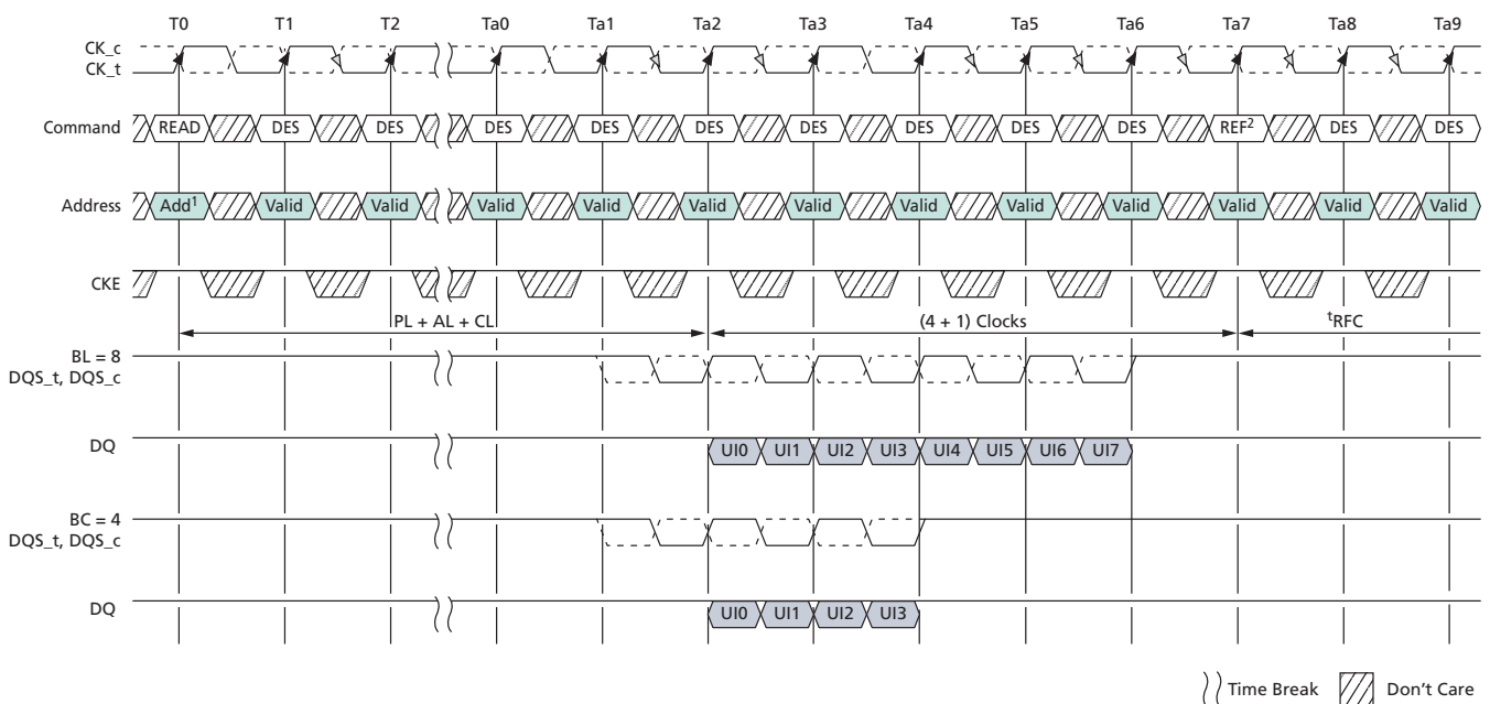
Figure 41: READ-to-REFRESH Timing
