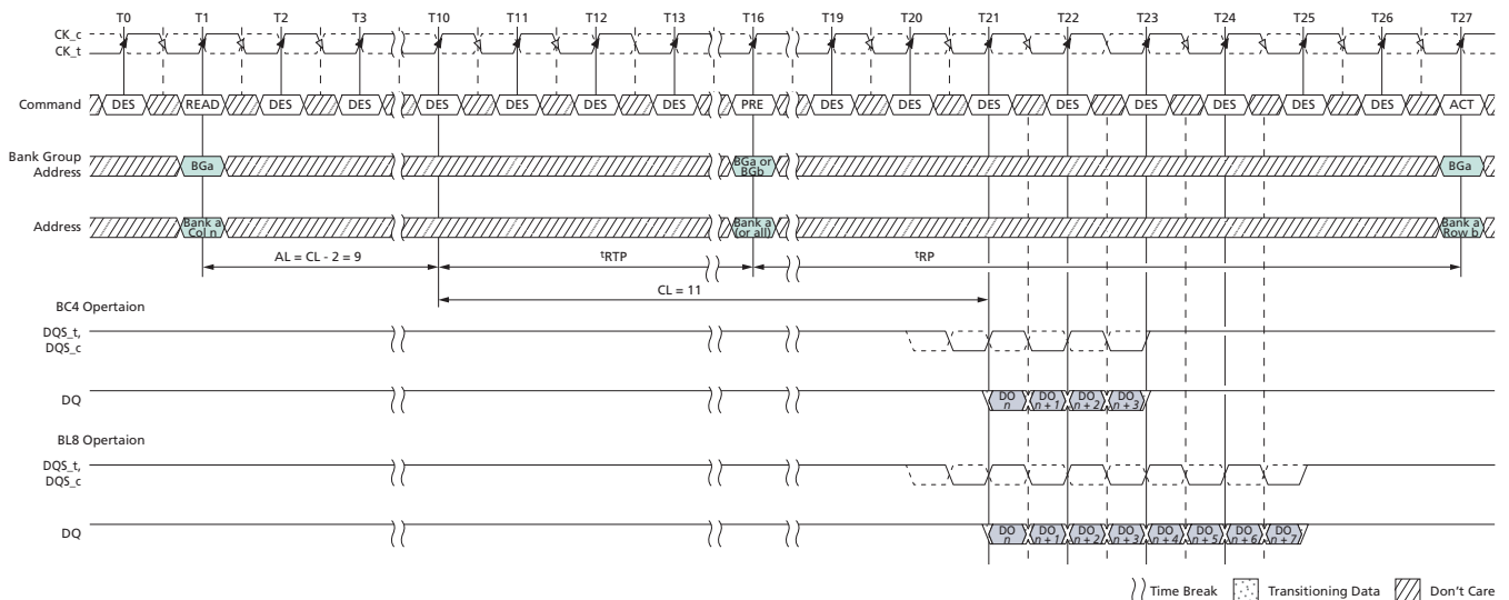
Figure 154: READ to PRECHARGE with Additive Latency and 1^t\text{CK} Preamble
