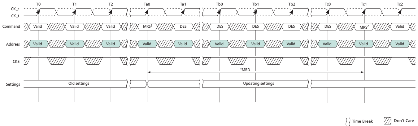
Figure 16: t^{\text{MRD}} Timing
