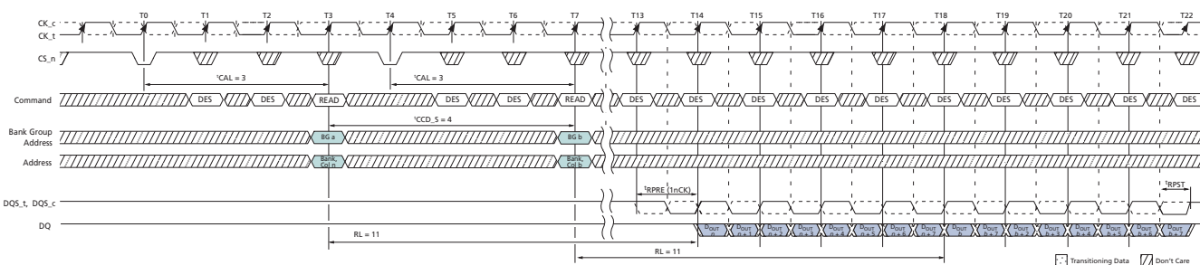
Figure 31: Consecutive READ BL8, CAL3, 1 st CK Preamble, Different Bank Group
