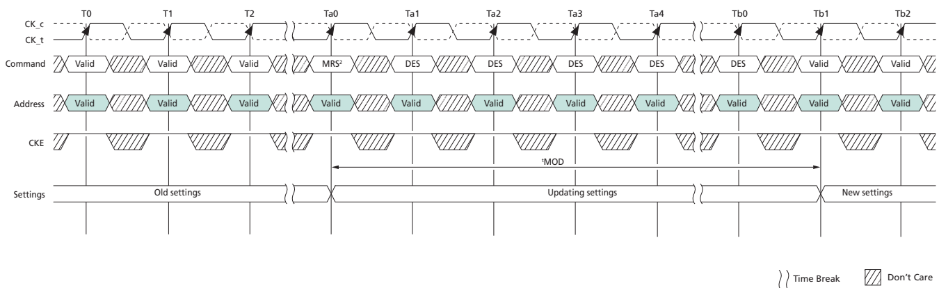
Figure 17: t^{\text{MOD}} Timing
