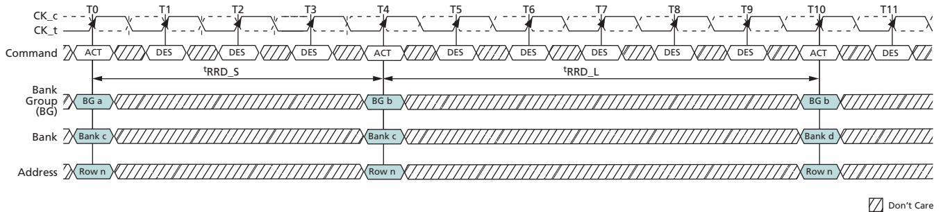
Figure 121: t^{\text{RRD}} Timing
