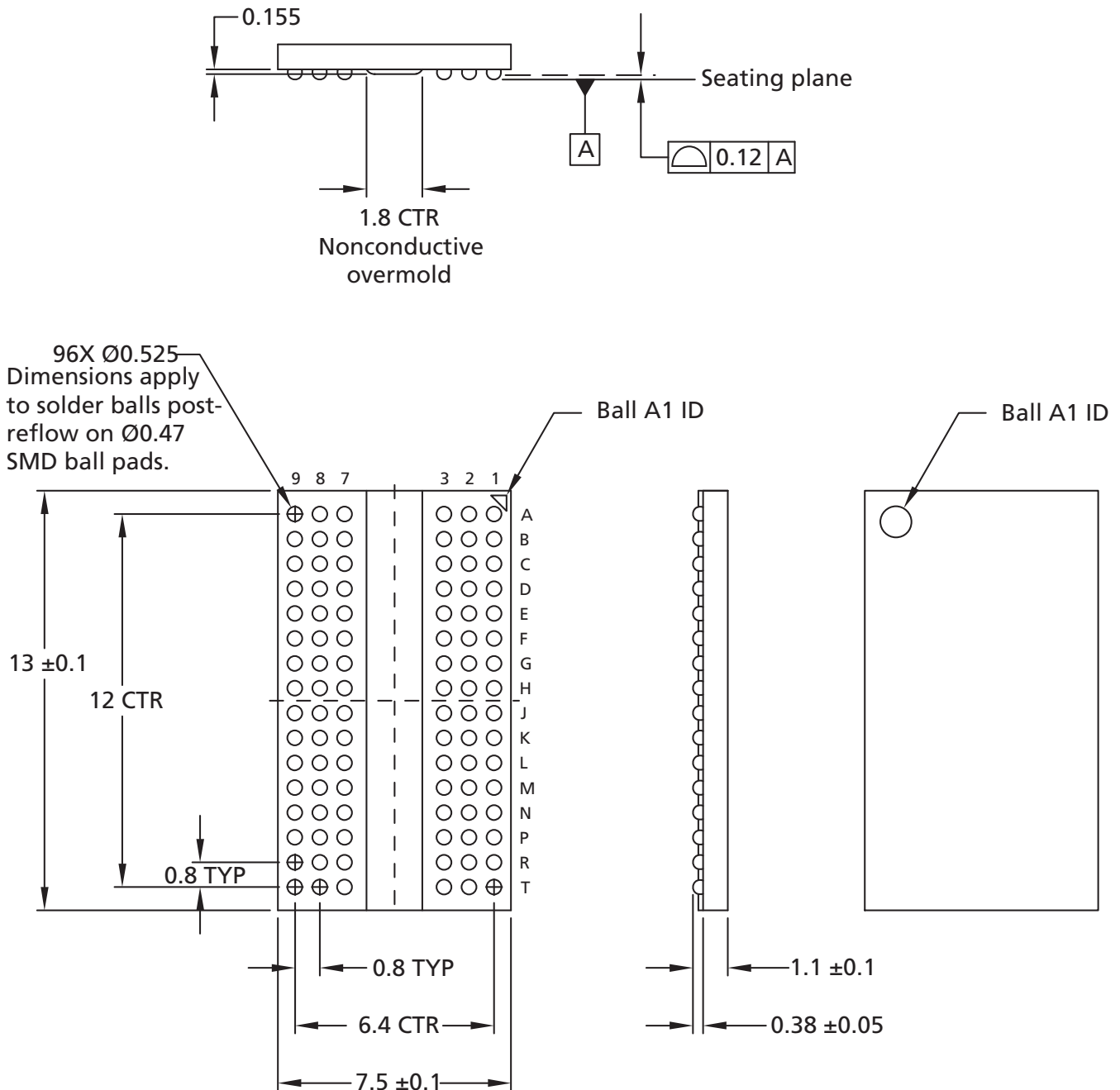
Figure 12: 96-Ball FBGA – x16 (TD)
