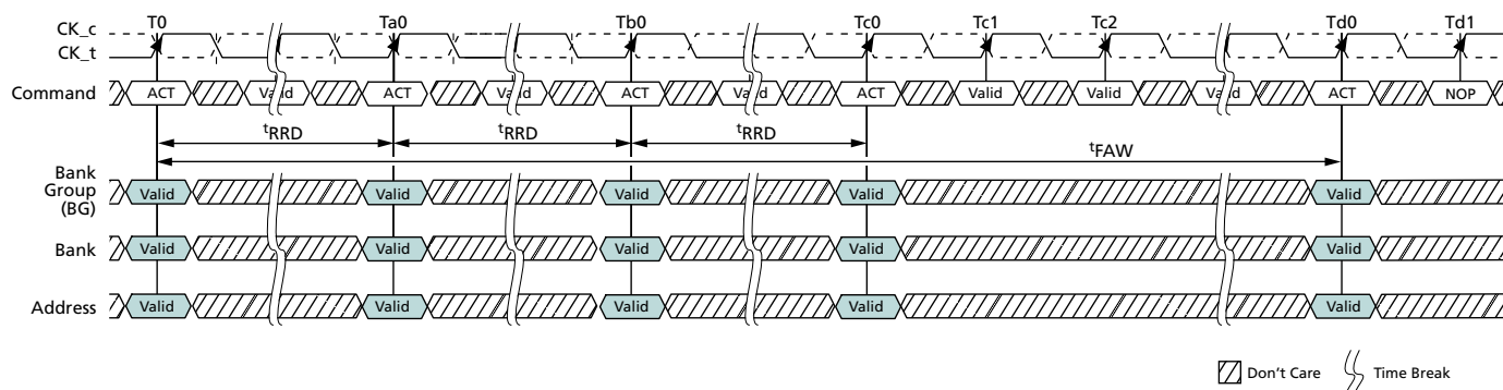
Figure 76: t_{FAW} Timing
