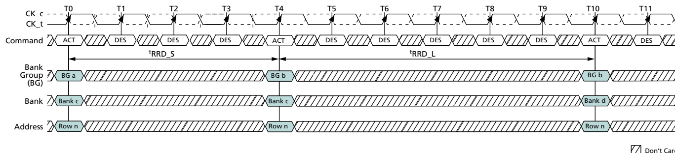
Figure 75: t_{RRD} Timing
