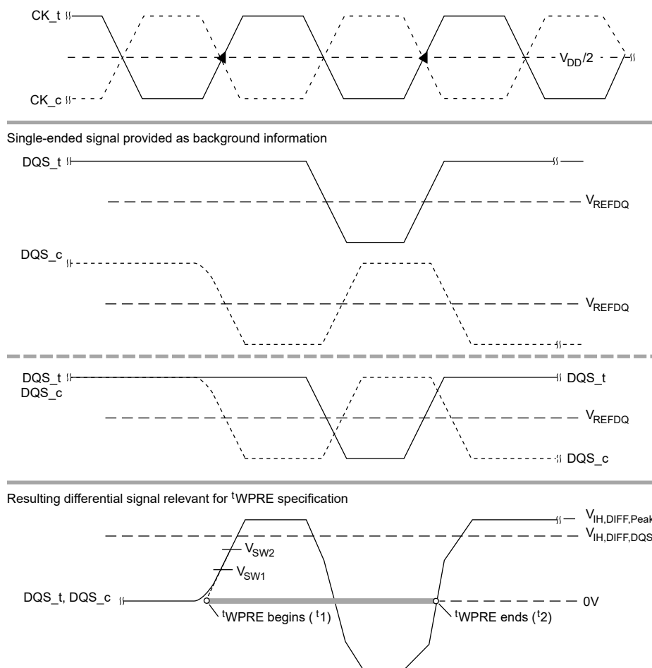
Figure 159: t_{WPRE} Method for Calculating Transitions and Endpoints
